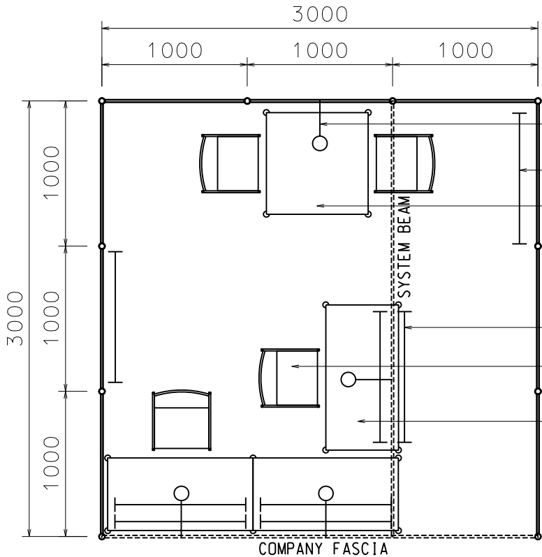
PLAN
